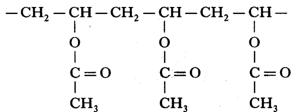
poly(ethenyl ethanoate)
